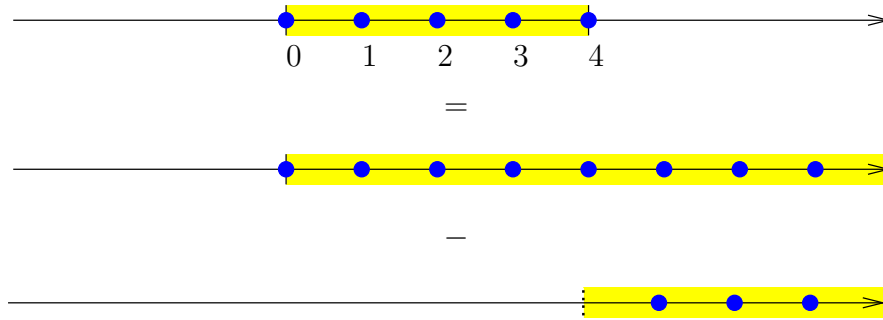
Figure 1.4: Another one-dimensional identity
