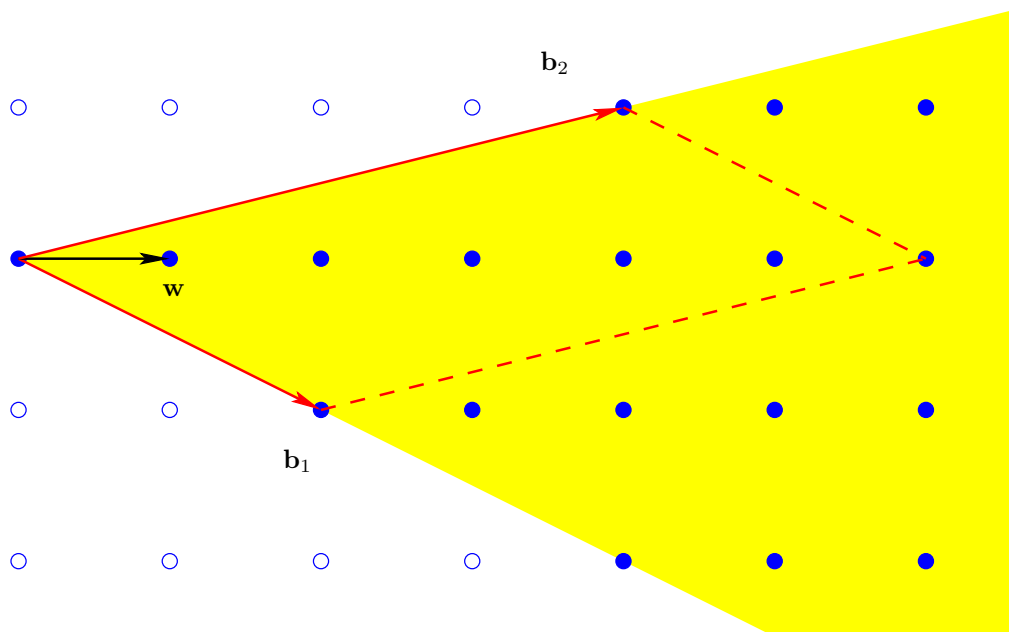
Figure 3.3: A two-dimensional cone of index 6 with its fundamental parallelepiped. Using the interior vector w , a triangulation can be constructed.
