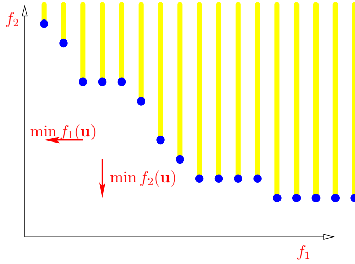
Figure 5.8: Outcome space, after erasing vertically dominated solutions
