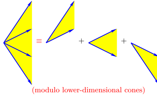
Figure 3.8: An identity, valid modulo lower-dimensional cones, corresponding to a polyhedral subdivision of a cone
