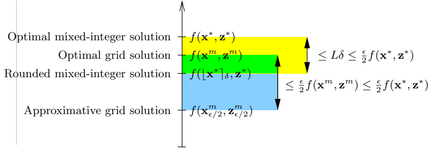
Figure 4.5: Estimates in the proof of Theorem 4.1 (a)
