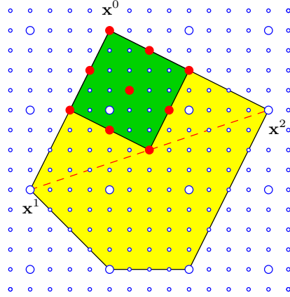
Figure 4.4: The geometry of Lemma 4.15 . For a polynomial with maximum total degree of 2, we construct a refinement \frac{1}{k}\mathbf{Z}^d (small circles) of the standard lattice (large circles) such that P \cap \frac{1}{k}\mathbf{Z}^d contains an affine image of the set \{0, 1, 2\}^d (large dots).
