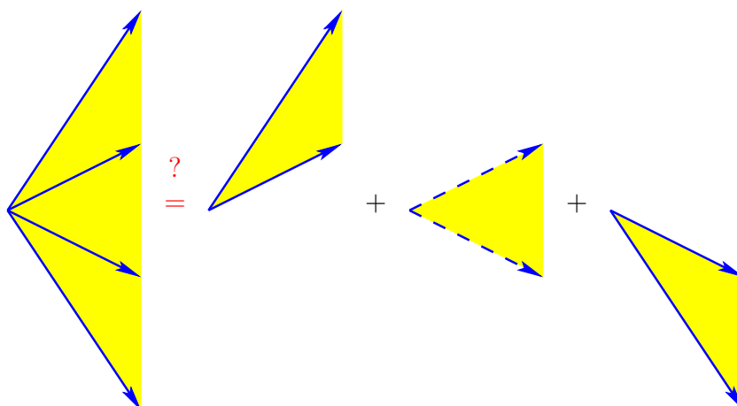
Figure 3.9: The technique of half-open exact decomposition. The above ad-hoc choice of strict inequalities (broken lines) and weak inequalities (solid lines) appears to give an exact identity on first look. However, the apex of the cone is still counted twice.
