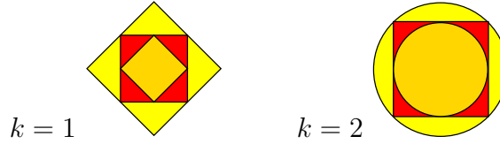
Figure 4.1: Approximation properties of \ell_k -norms
