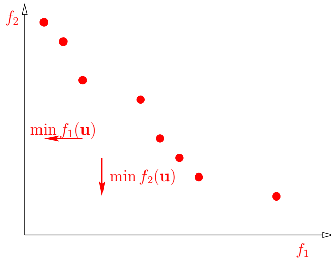
Figure 5.9: Outcome space, after erasing all dominated solutions
