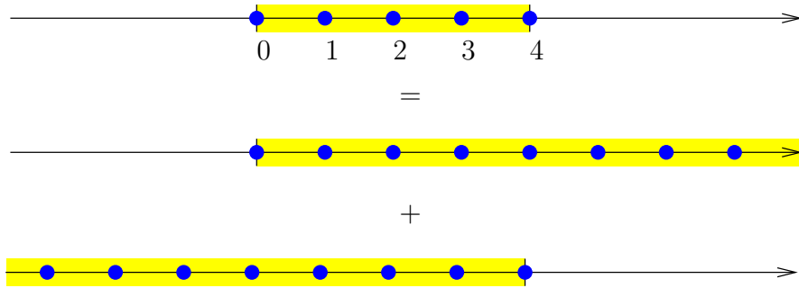
Figure 1.2: One-dimensional Brion theorem
