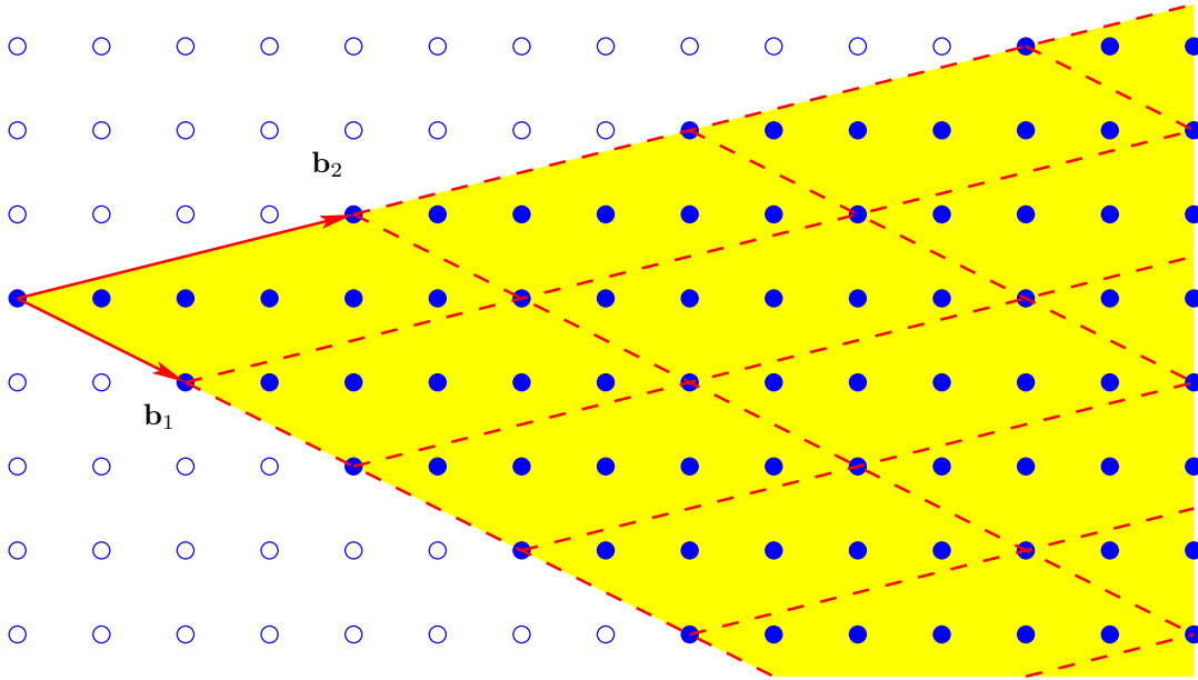
Figure 3.1: Tiling a rational two-dimensional cone with copies of the fundamental parallelepiped
