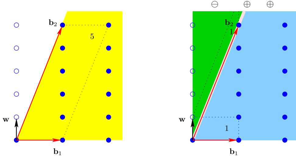
Figure 3.6: A signed decomposition of the cone of index 5 generated by \mathbf{b}^1 and \mathbf{b}^2 into the two unimodular cones spanned by \{\mathbf{b}^1, \mathbf{w}\} and \{\mathbf{b}^2, \mathbf{w}\} . We have the inclusion-exclusion formula g(\text{cone}\{\mathbf{b}_1, \mathbf{b}_2\}; \mathbf{z}) = g(\text{cone}\{\mathbf{b}_1, \mathbf{w}\}; \mathbf{z}) - g(\text{cone}\{\mathbf{b}_2, \mathbf{w}\}; \mathbf{z}) + g(\text{cone}\{\mathbf{w}\}; \mathbf{z}) .
