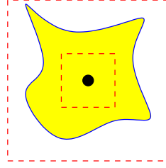
Figure 5.10: A set defining a pseudo-norm with the inscribed and circumscribed cubes \alpha B_\infty and \beta B_\infty (dashed).
