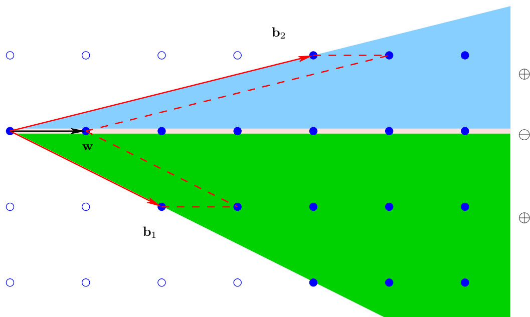
Figure 3.4: A two-dimensional cone of index 6, triangulated into two unimodular cones. The integer points in the one-dimensional intersection would be counted twice, so we subtract them once (inclusion–exclusion principle).
