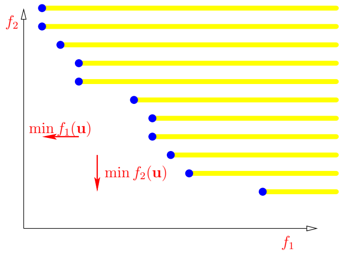
Figure 5.7: Outcome space, after erasing horizontally dominated solutions
