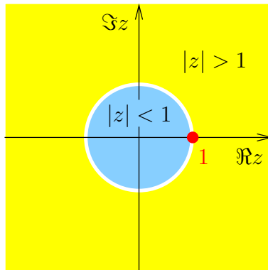
Figure 1.3: The domains of convergence of the Laurent series
