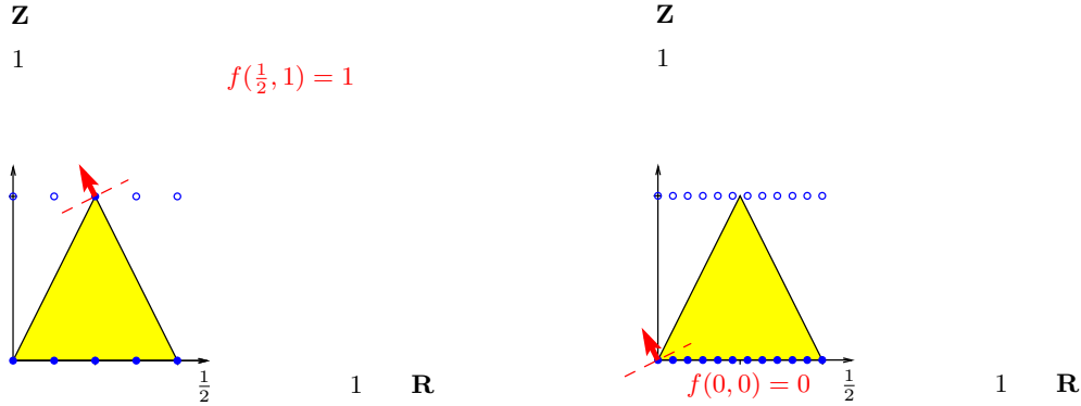
Figure 4.2: A sequence of optimal solutions to grid problems with two limit points, for even m and for odd m
