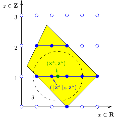
Figure 4.3: The principle of grid approximation. Since we can refine the grid only in the direction of the continuous variables, we need to construct an approximating grid point (\mathbf{x}, \mathbf{z}^*) in the same integral slice as the target point (\mathbf{x}^*, \mathbf{z}^*) .
