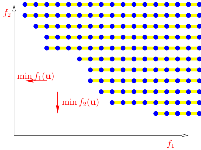
Figure 5.6: Outcome space, epigraph
