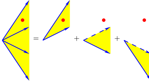
Figure 3.10: The technique of half-open exact decomposition. The relative location of the vector \mathbf{y} (represented by a dot) determines which defining inequalities are strict (broken lines) and which are weak (solid lines).
