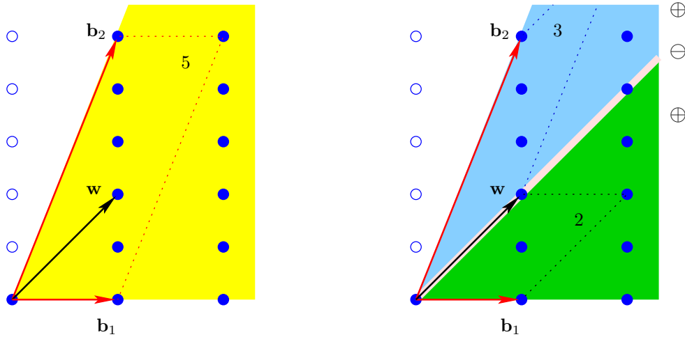
Figure 3.5: A triangulation of the cone of index 5 generated by \mathbf{b}^1 and \mathbf{b}^2 into the two cones spanned by \{\mathbf{b}^1, \mathbf{w}\} and \{\mathbf{b}^2, \mathbf{w}\} , having an index of 2 and 3, respectively. We have the inclusion-exclusion formula g(\text{cone}\{\mathbf{b}_1, \mathbf{b}_2\}; \mathbf{z}) = g(\text{cone}\{\mathbf{b}_1, \mathbf{w}\}; \mathbf{z}) + g(\text{cone}\{\mathbf{b}_2, \mathbf{w}\}; \mathbf{z}) - g(\text{cone}\{\mathbf{w}\}; \mathbf{z}) ; here the one-dimensional cone spanned by \mathbf{w} needed to be subtracted.
