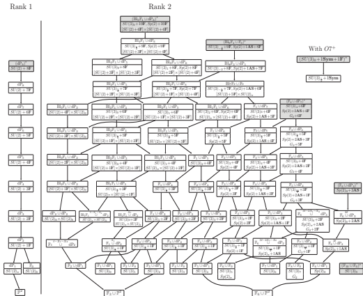
Figure 10. The diagram above shows the RG flow among rank 1 and rank 2 SCFTs obtained by mass deformations. The first and the second rows in each box correspond to the geometric and the gauge theoretic descriptions respectively of a 5d theory. The parent theory in each branch is a 5d KK theory related to a 6d theory on S^1 .
