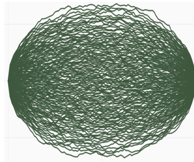
Gibbsian line ensembles
