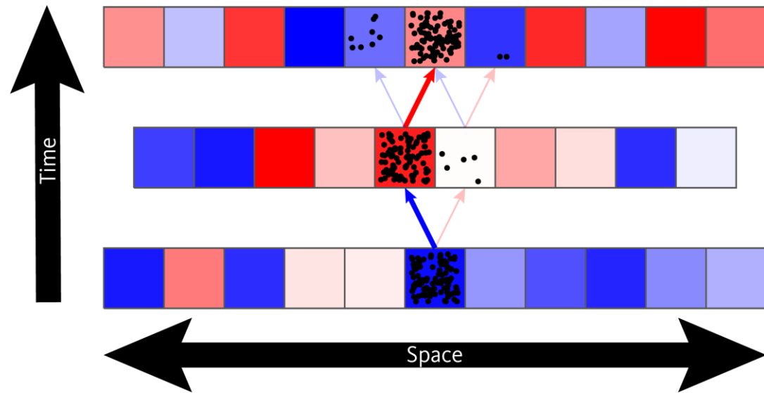
Space-time RWRE
