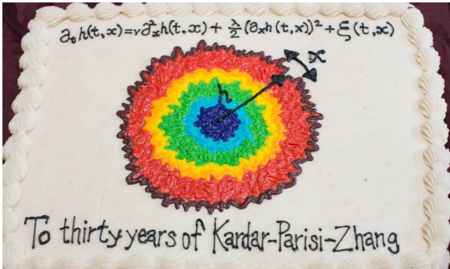
Kardar-Parisi-Zhang growth
