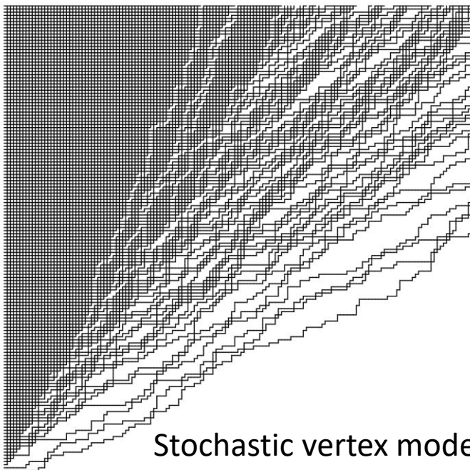
Kardar-Parisi-Zhang growth
