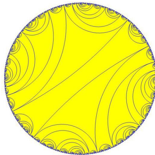
Invariant laminations
