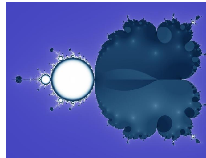
The parameter space of complex cubic polynomials
