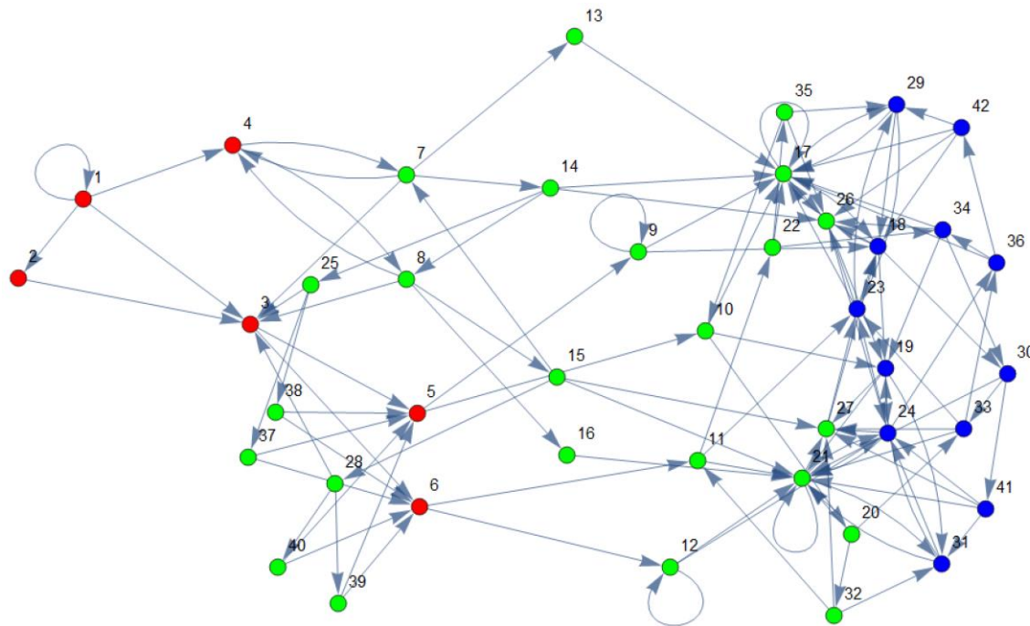
Polynomial renormalization
