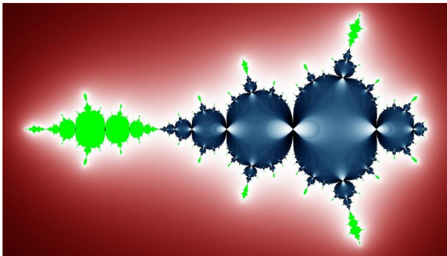
Polynomial renormalization
