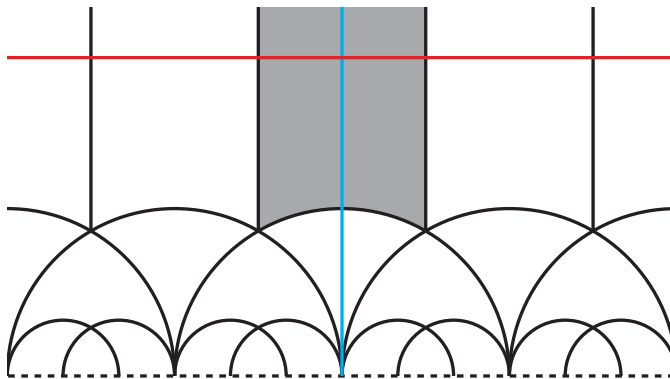
FIGURE 1. Fundamental domain for the action of SL_2(\mathbb{Z}) on \mathbb{H} in gray.
